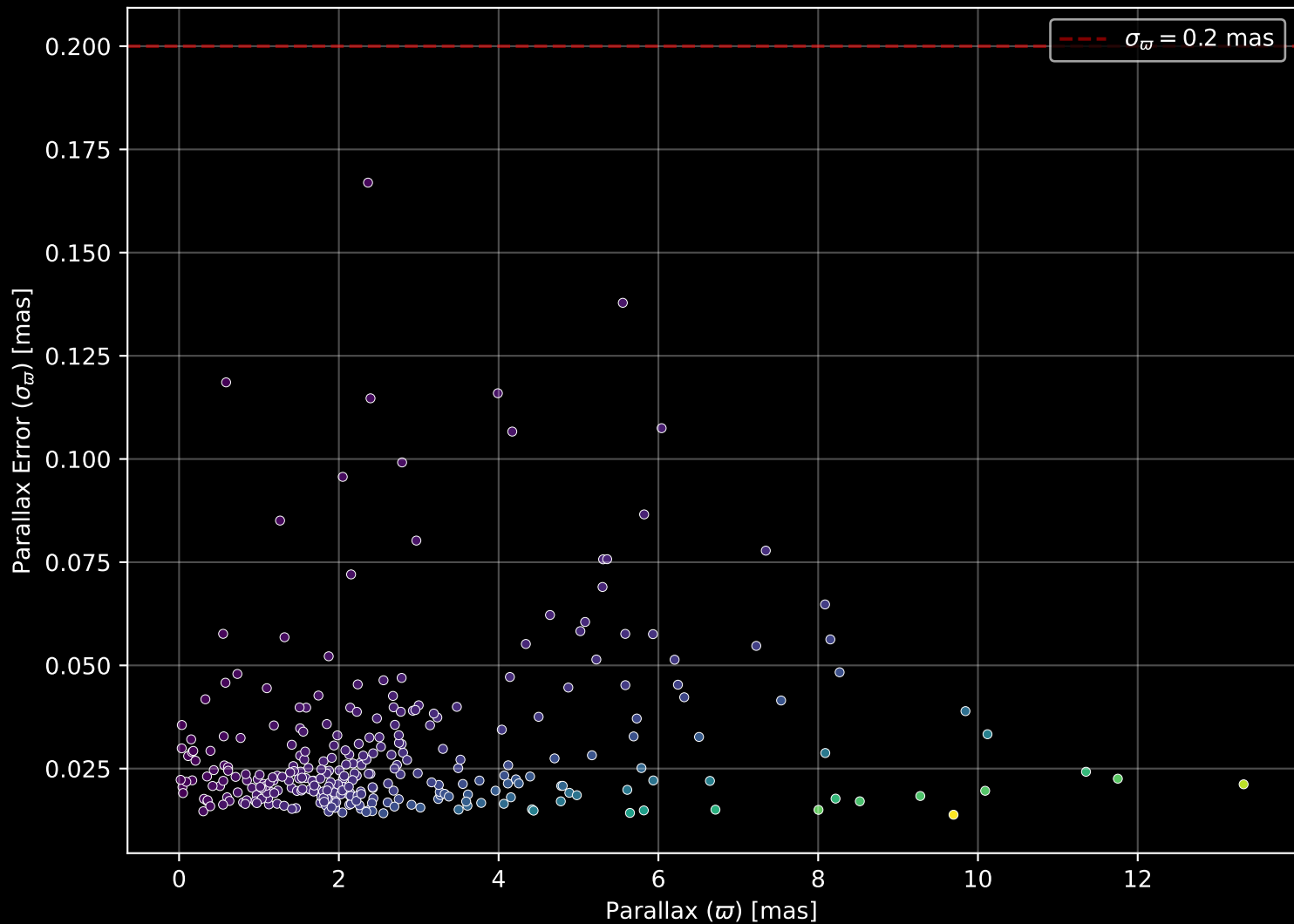
APOGEE DR17 Field: [060-72] Parallax Quality (n= 307)
