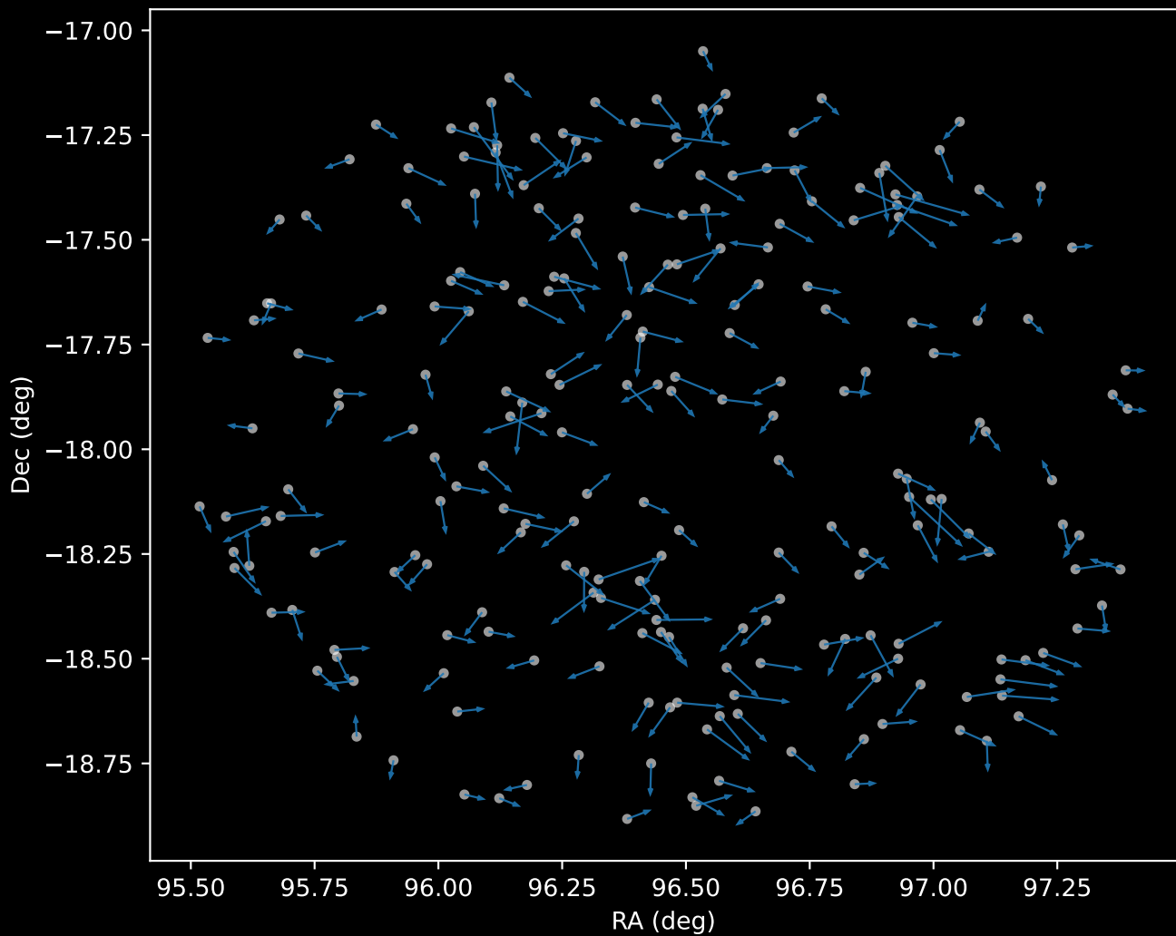
APOGEE DR17 Cluster 0 Proper Motion Vectors (n=227)
