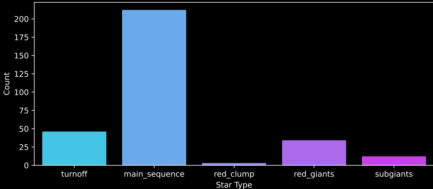
APOGEE DR17 Field: [060-72] Count plot of Star Type
