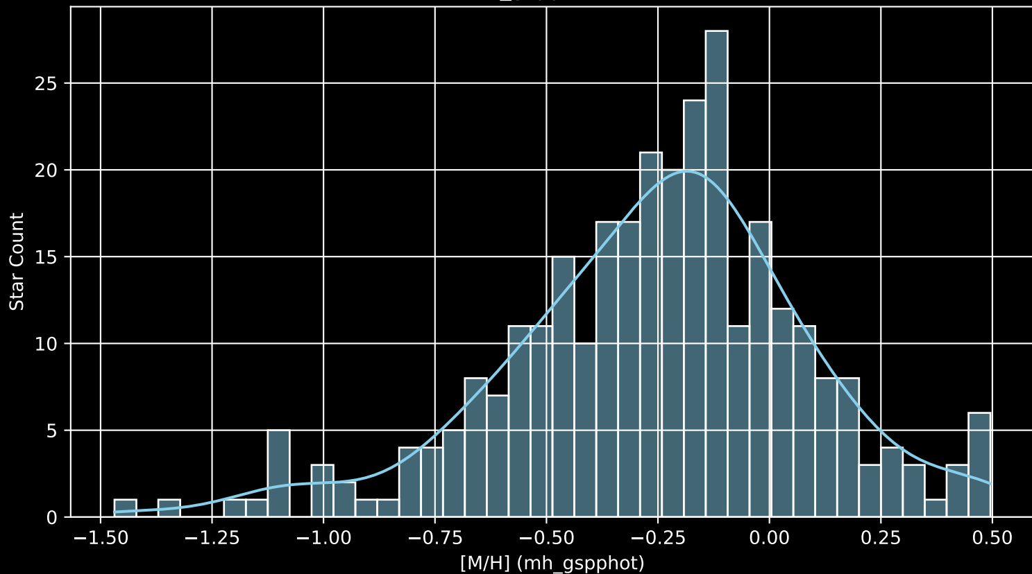
APOGEE DR17 Field: [060-72 [M/H] (mh_gspphot) (n= 305)
