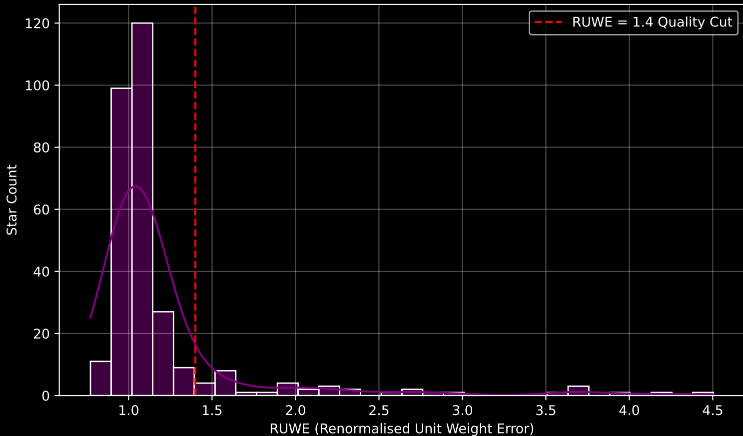
GAPOGEE DR17 Field [060-72] RUWE Distribution (n= 303)
