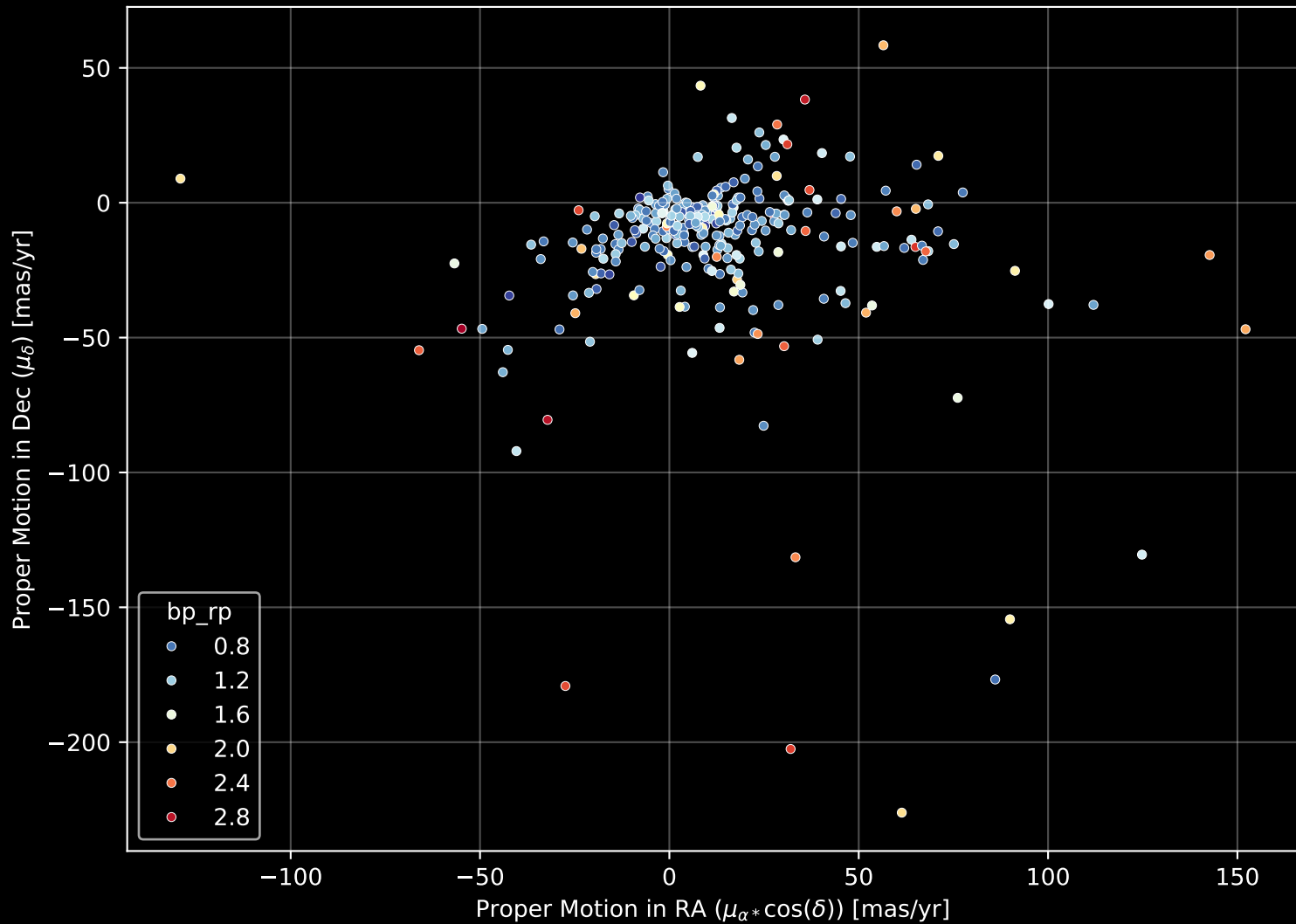
APOGEE DR17 Field: [060-72] Proper Motion Diagram (n= 307)
