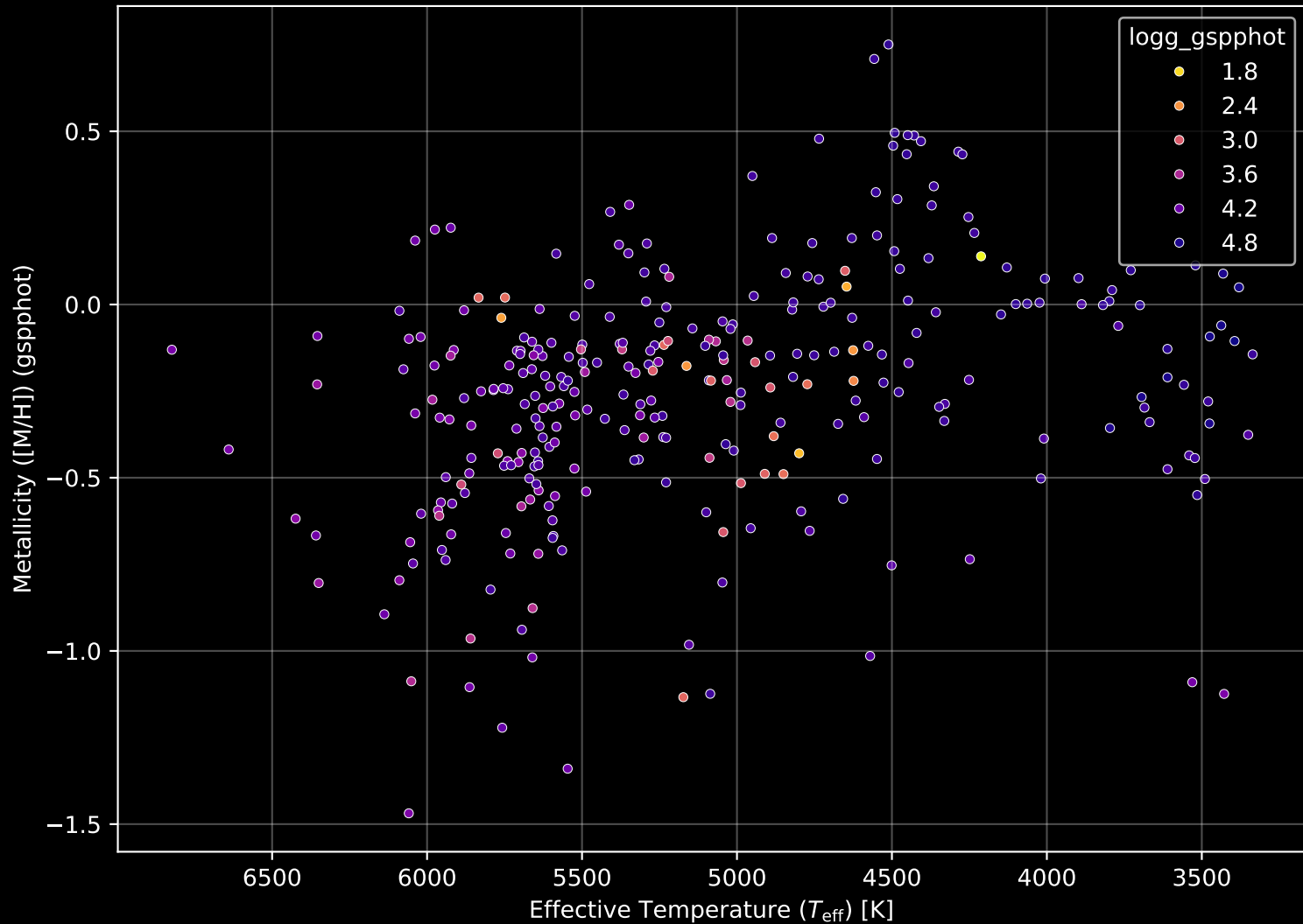
APOGEE DR17 Field: [060-72] Stellar Population Parameters (n= 307)
